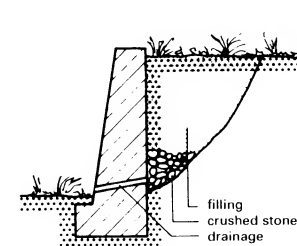
27 Concrete retaining wall (also available in ready-made sections) -> 28
